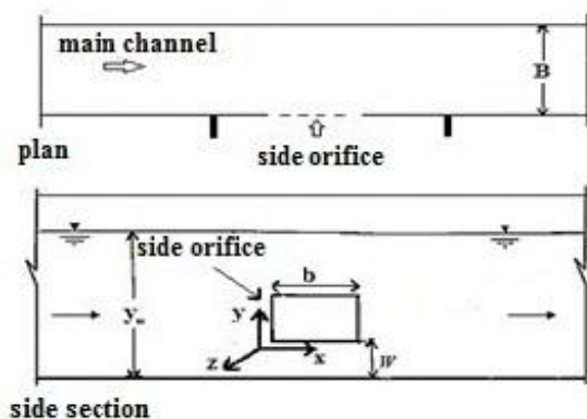
Fig. 1. Plan and side section of the main channel
