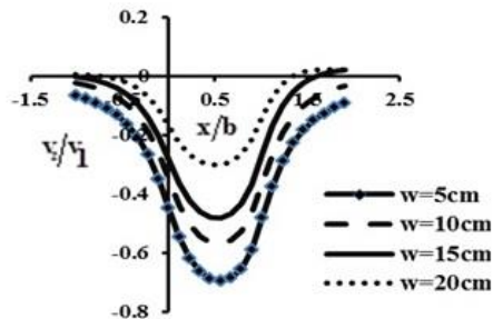
Fig. 10. The non-dimensional vertical velocity distribution close to the orifice section at the level a) 0.25 and b) 0.75 of the orifice height for different heights of the side orifices crest
