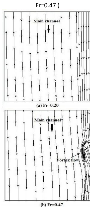
Fig. 5.The streamline patterns near free surface around the orifice for a) Fr=0.20 and b) Fr=0.47
