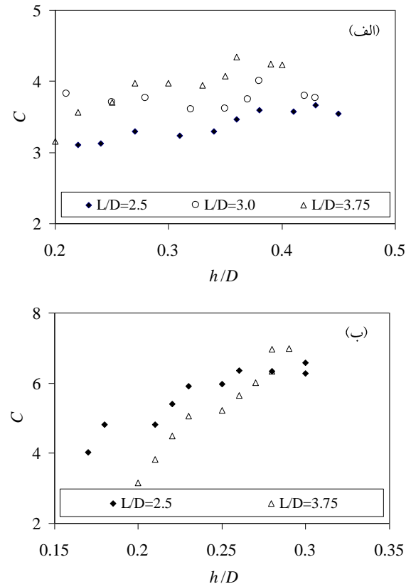
Figure (9) Discharge coefficient versus h/D for P/D=1 , for marguerite spillways with a- two blades and b- three blades
