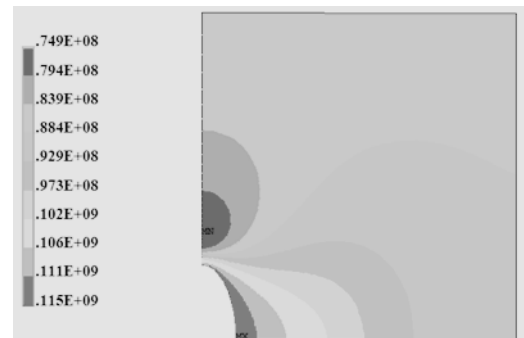
Fig. 13. von Mises stress distribution over the optimized hole using evolutionary structural optimization and nonlinear analysis
